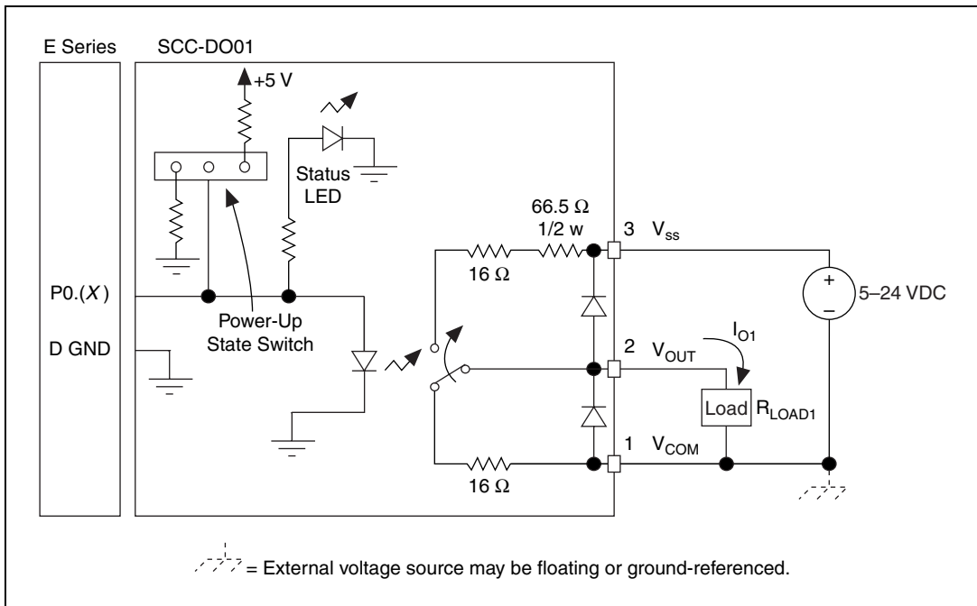
Figure 1. Connecting a Load R_{LOAD1} to V_{COM} and V_{OUT} (Configuration 1)
